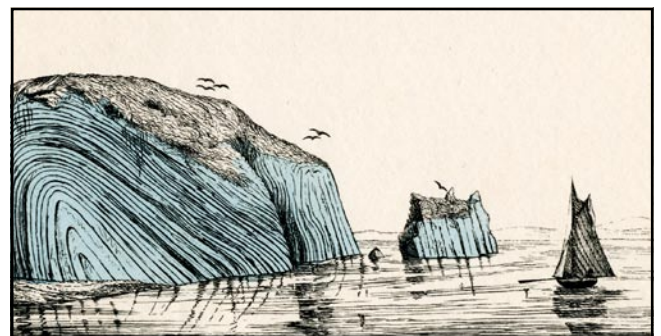
Figure 10. Sketch by De la Beche showing folded Carboniferous Limestone near Torquay, south Devon (from Transactions of the Geological Society, 1829).
